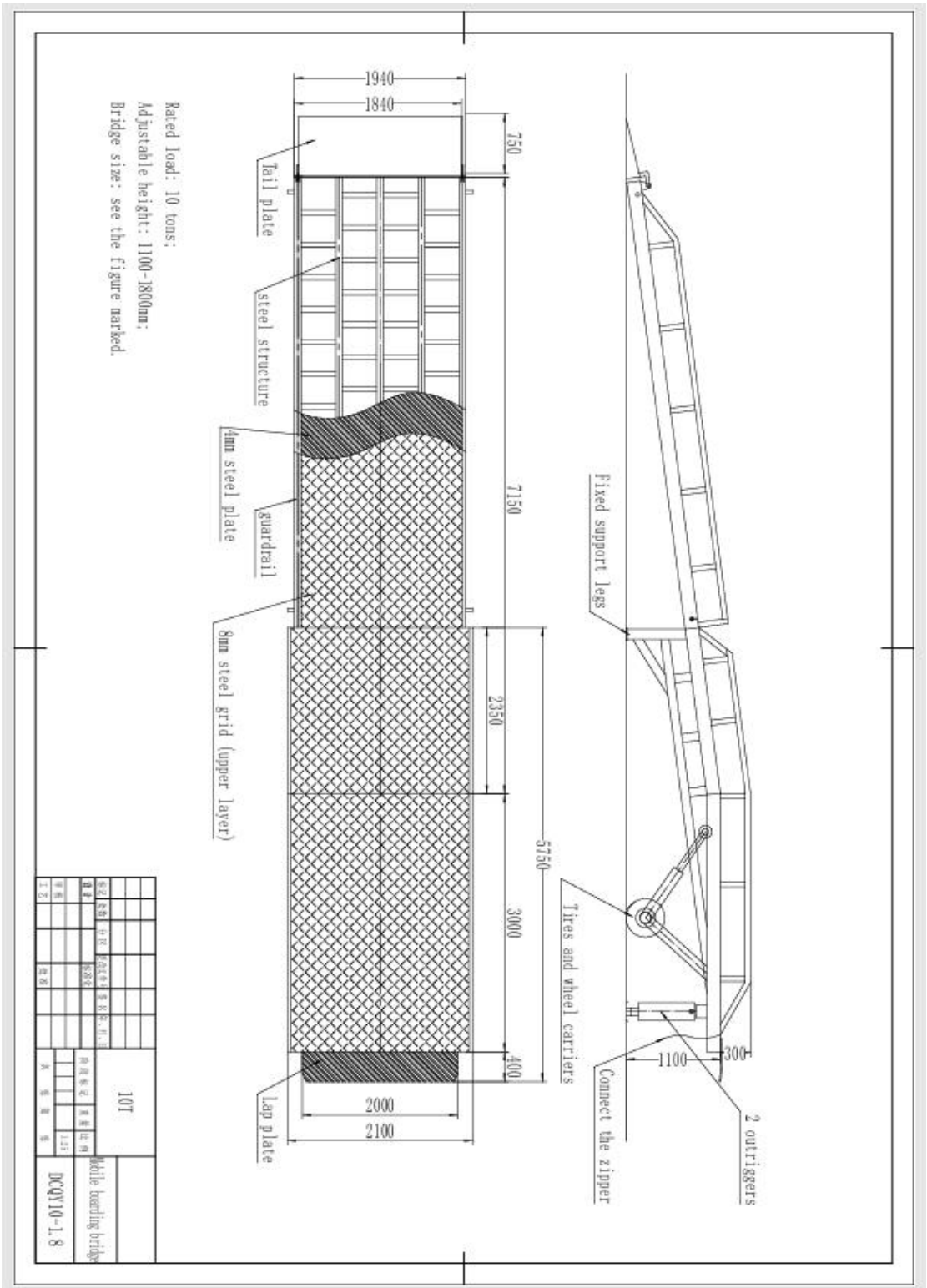
10-ton foldable mobile loading and unloading ramp configuration drawing:
